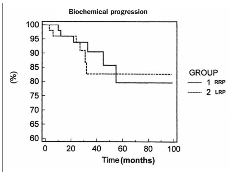
Figure 1. Kaplan Meier curves for biochemical progression.
