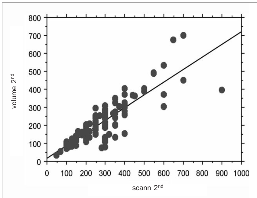
Figure 2. Linear regression analysis yielded 2 nd flow rate recording is \text{Void-Vol} = 16.264 + (0.704 * \text{Pre-Vol}) ( r = 0.855 ; p < 0.0001 ).
